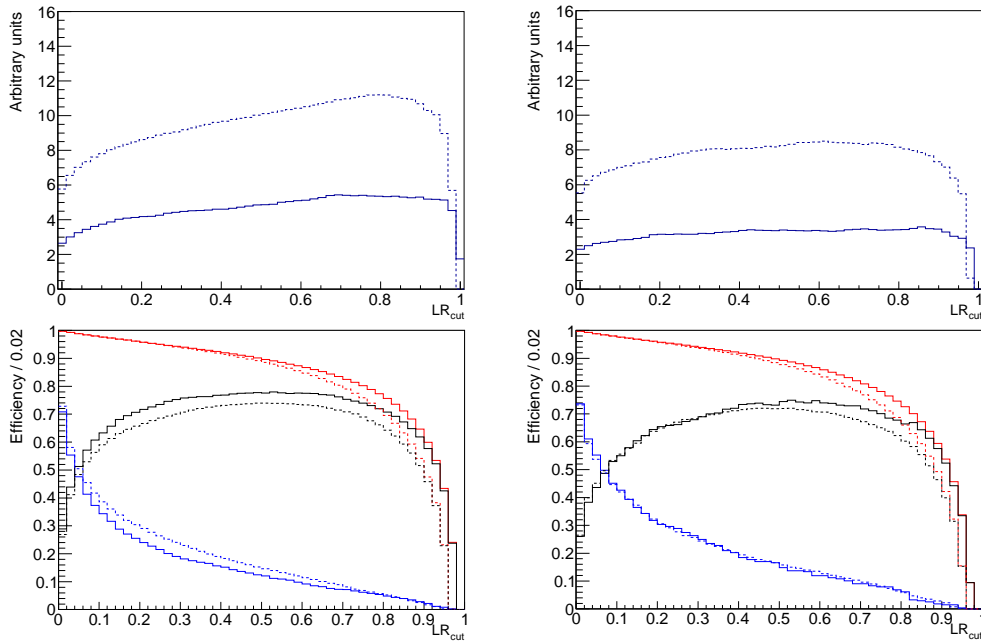
Fig. 3.7: F.O.M. (top) and calculated efficiencies (bottom) for the charged mode (left) and the neutral mode (right). The solid line shows results for SVD1 experiment, dashed line for SVD2 experiment. The red line describes signal efficiencies, blue line background efficiencies and black line the difference of signal and background efficiencies; all expressed with respect to the applied \mathcal{LR} ( \mathcal{CS}_{\text{cut}} ).
