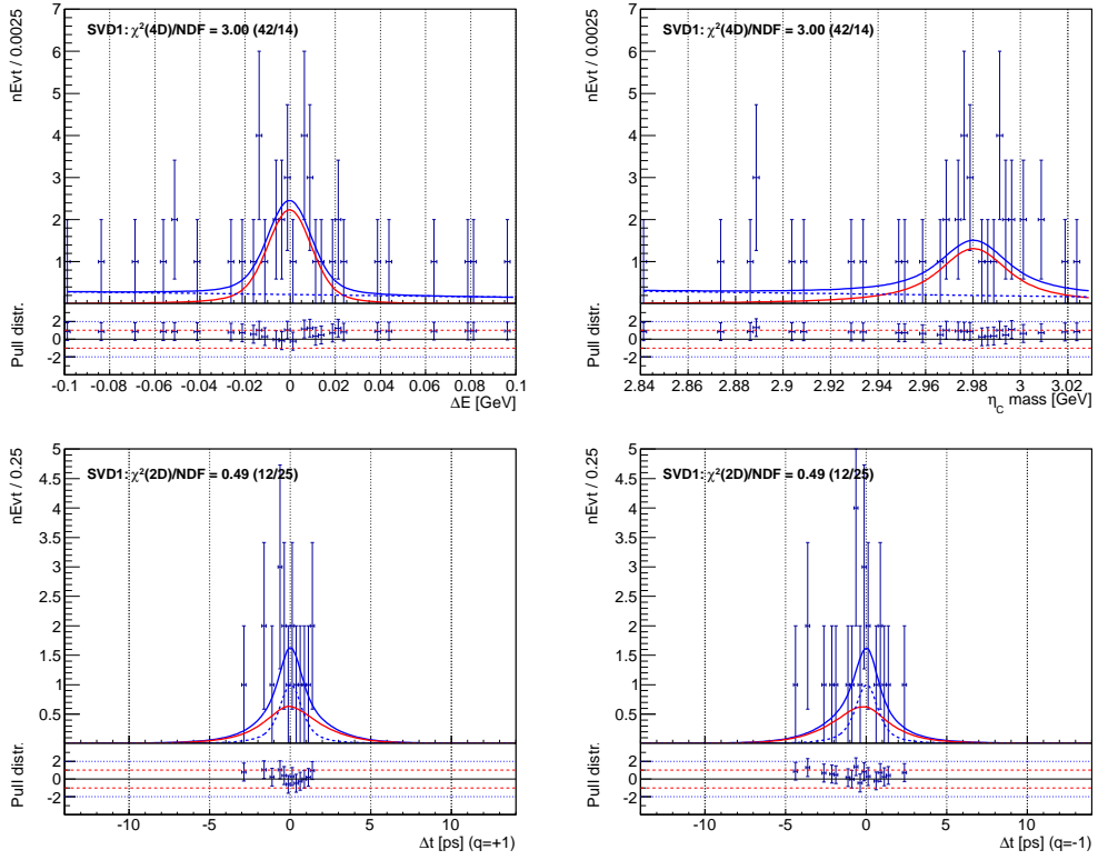
Fig. 7.2: Fit projections for SVD1 experiment in B^0 \rightarrow \eta_c K_S^0 , \eta_c \rightarrow p\bar{p} : \Delta E (top left), \eta_c invariant mass (top right), \Delta t for B tagged with q = +1 (down left) and \Delta t for B tagged with q = -1 (down right). The red curve represents a signal PDF, dashed blue curve a background PDF and solid blue line a sum of both.
