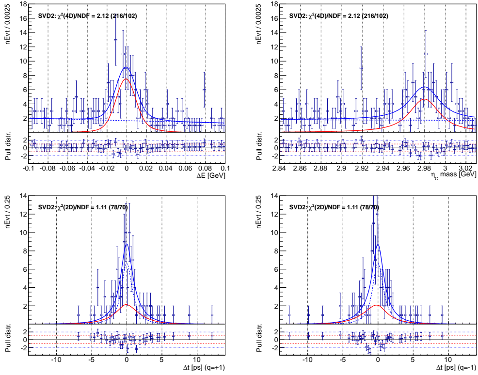
Fig. 7.3: Fit projections for SVD2 experiment in B^0 \rightarrow \eta_c K_S^0 , \eta_c \rightarrow p\bar{p} : \Delta E (top left), \eta_c invariant mass (top right), \Delta t for B tagged with q = +1 (down left) and \Delta t for B tagged with q = -1 (down right). The red curve represents a signal PDF, dashed blue curve a background PDF and solid blue line a sum of both.
