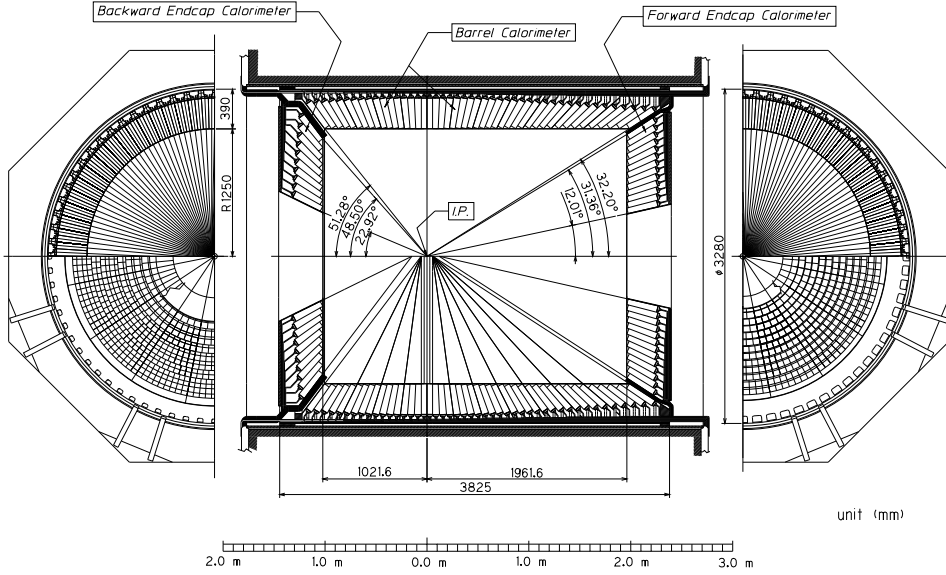
Fig. 2.10: Overall geometry layout of the Electromagnetic CaLorimeter [21].
