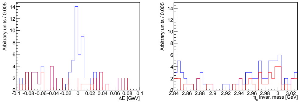
Fig. 3.8: \Delta E (left) and \eta_c invariant mass distribution obtained from the generic b\bar{b} MC study, before (blue) and after (red) application of m(\bar{p}K_S^0) veto.
