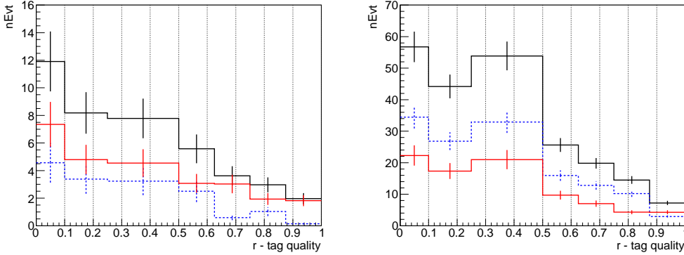
Fig. 7.1: Number of fit events versus tag quality, r , ( r -bin fractions) for SVD1 (left) and SVD2 (right) experiment. The number of signal (background) events is represented by solid red (dashed blue) curve, the sum of both contributions by solid black curve.
