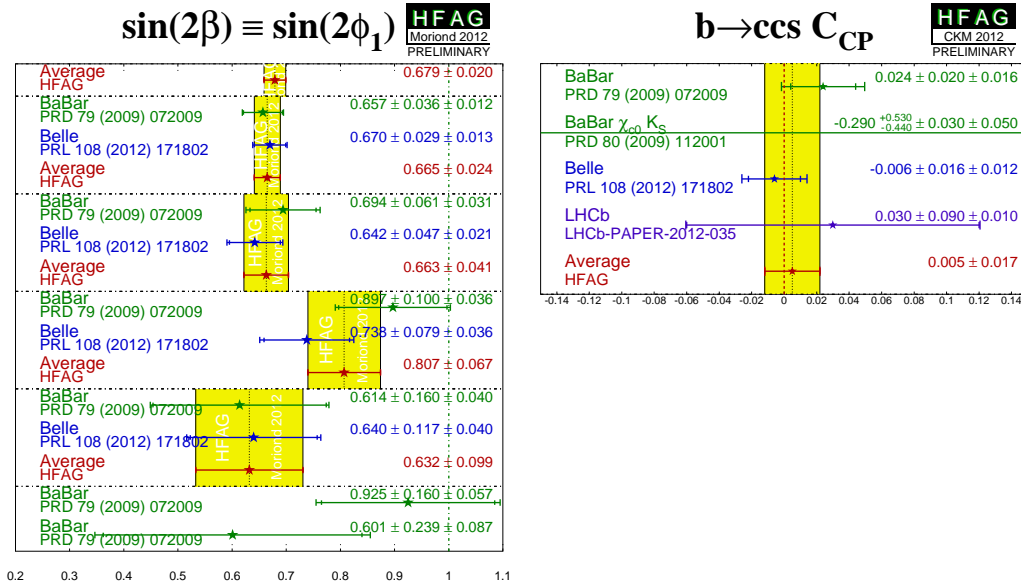
Fig. 8.1: Current average of \sin 2\phi_1 \equiv \mathcal{S}_{CP} (left) and C \equiv -\mathcal{A}_{CP} (right) by B -factories [18]. The left plot lists the following B decay measurements: world average with all channels included, J/\psi K_S^0 , J/\psi K_L^0 , \psi(2S)K_S^0 , \chi_{c1}K_S^0 , \eta_c K_S^0 and J/\psi K^{*0} ( K^{*0} \rightarrow K_S^0 \pi^0 ) by BaBar only.
