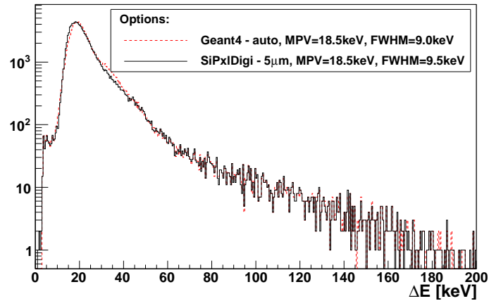
Figure 4: Comparison of energy loss fluctuations by 0.5 GeV/c pions in 80 \mu\text{m} thick silicon generated at Geant4 level, with \text{MPV} = 18.5 \text{ keV} and \text{FWHM} = 9.0 \text{ keV} (red dashed line), versus digitization level, with \text{MPV} = 18.5 \text{ keV} and \text{FWHM} = 9.5 \text{ keV} (black solid line). To emphasize agreement in distribution tails, log-scale is used.
