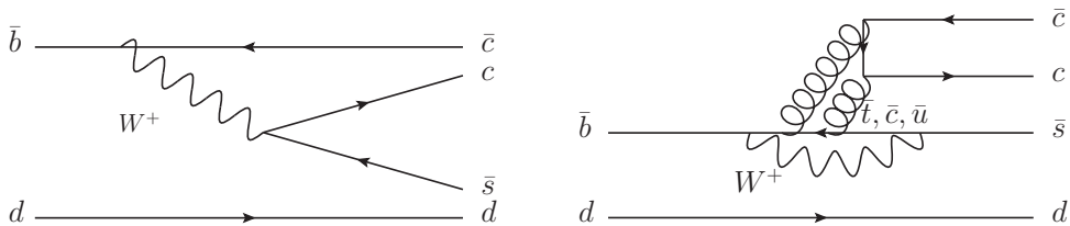
Fig. 1.1: Tree and penguin diagrams for b \rightarrow c\bar{c}s induced decays, such as B^0 \rightarrow J/\psi K_S^0 (with 3-gluon exchange in the penguin graph) or B^0 \rightarrow \eta_c K_S^0 .
