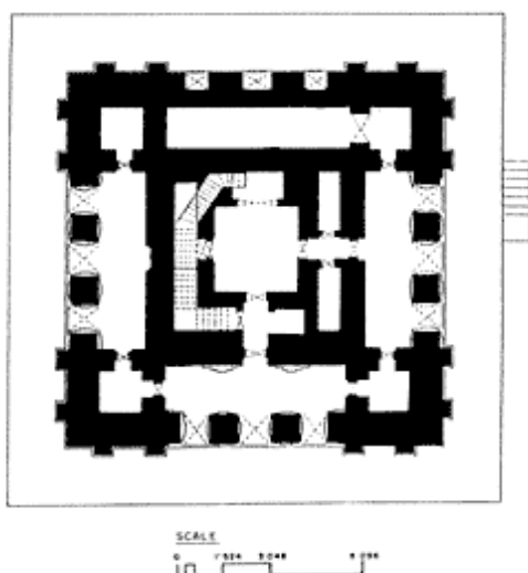
PLAN OF RADHA GOVINDA TEMPLE BISHNUPUR
