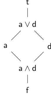
Figure 8.2: The algebra \mathbf{DM}_6
