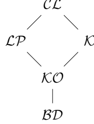
Figure 8.3: Super-Belnap logics with the proof by cases property
